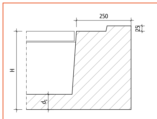
Detail-A1
