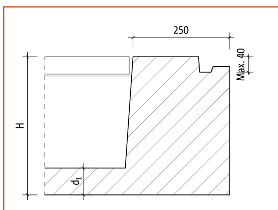
Detail-A2
