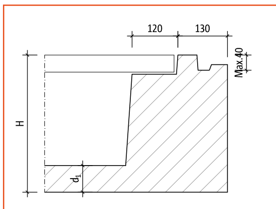
Detail-C2
